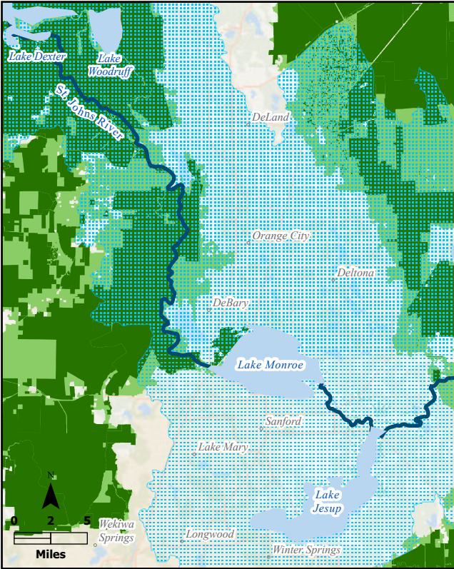
Lake Monroe, the St. Johns River, Contiguous Watersheds, and the Florida Wildlife Corridor
